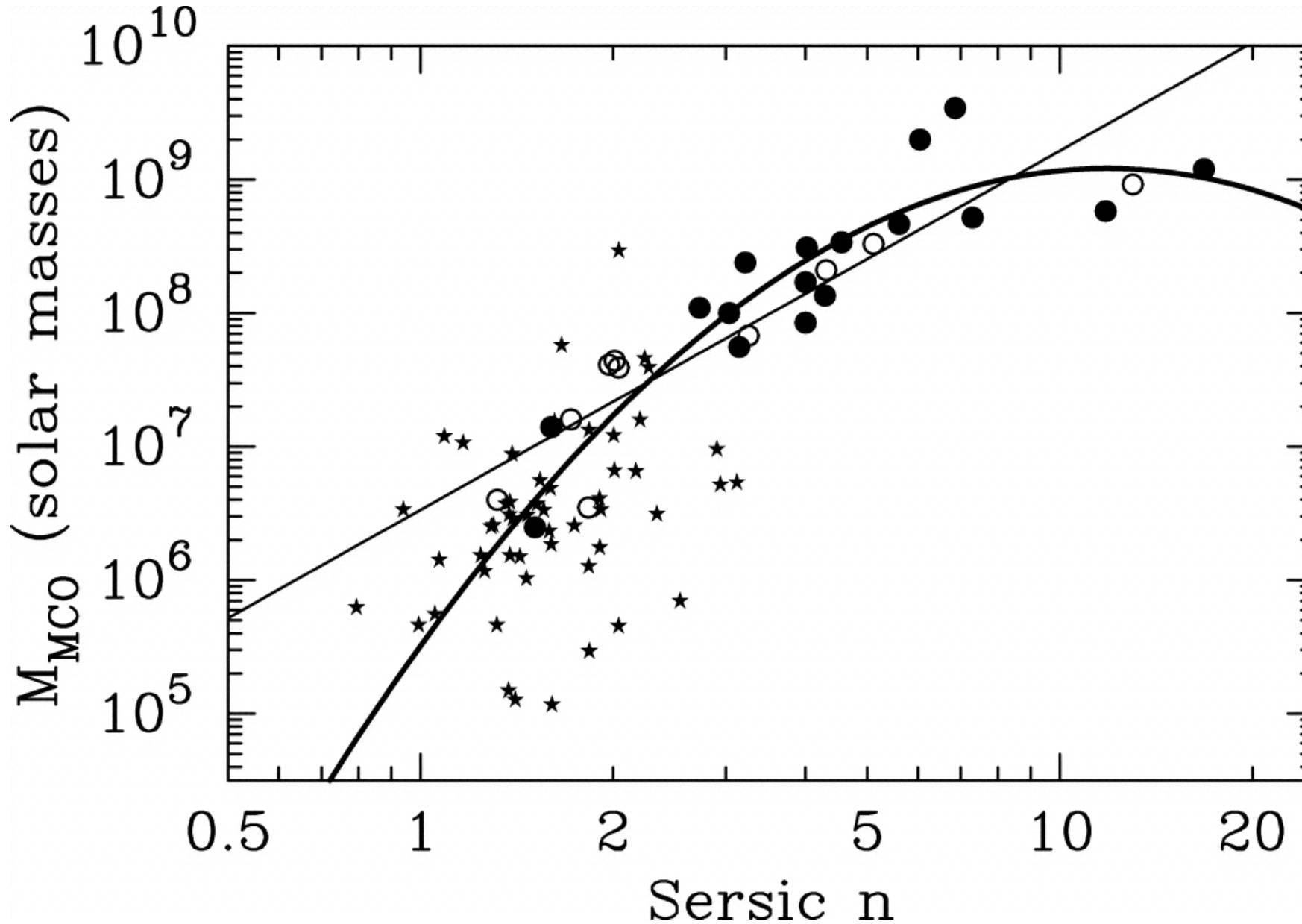
Fig. 3. from A LogQuadratic Relation for Predicting Supermassive Black Hole Masses from the Host Bulge Sérsic Index Graham & Driver 2007 ApJ 655 77 doi:10.1086/509758 https://dx.doi.org/10.1086/509758 © 2007. The American Astronomical Society. All rights reserved. Printed in U.S.A.
