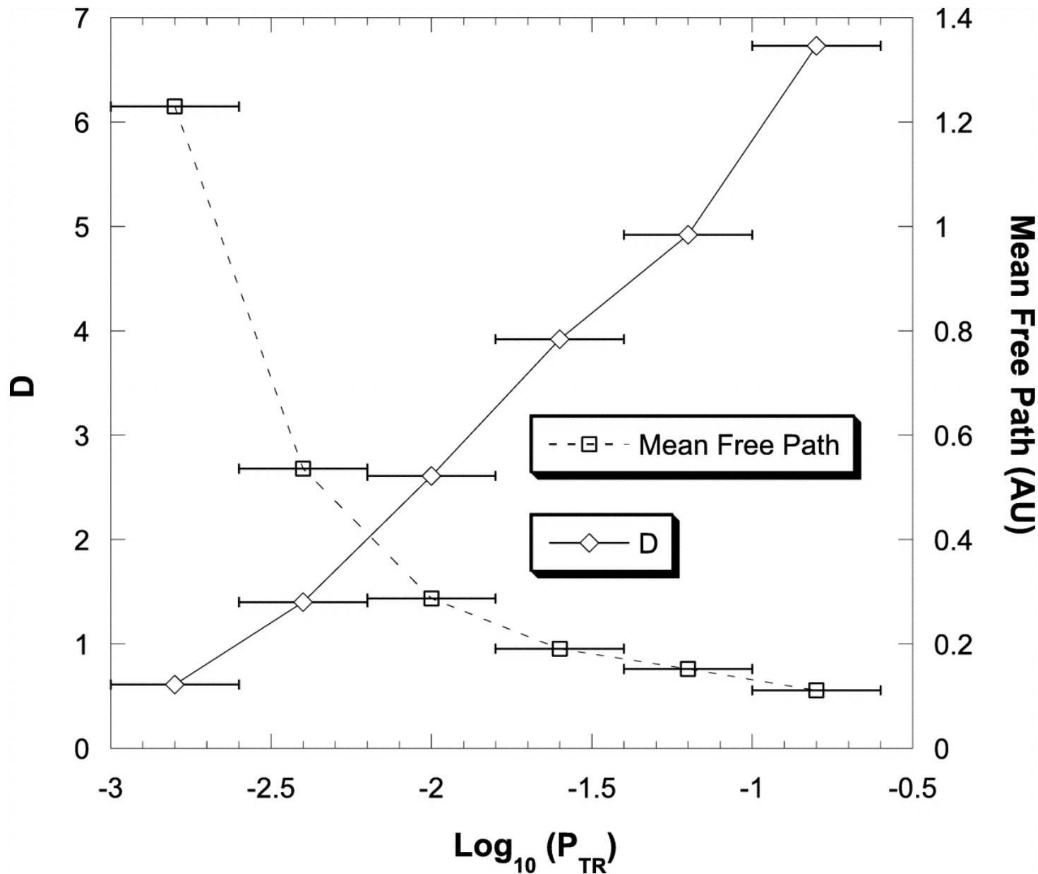
Fig. 6. from On PitchAngle Scattering Rates of Interstellar Pickup Ions as Determined by in Situ Measurement of Velocity Distributions Saul et al. 2007 ApJ 655 672 doi:10.1086/509732 https://dx.doi.org/10.1086/509732 © 2007. The American Astronomical Society. All rights reserved. Printed in U.S.A.
