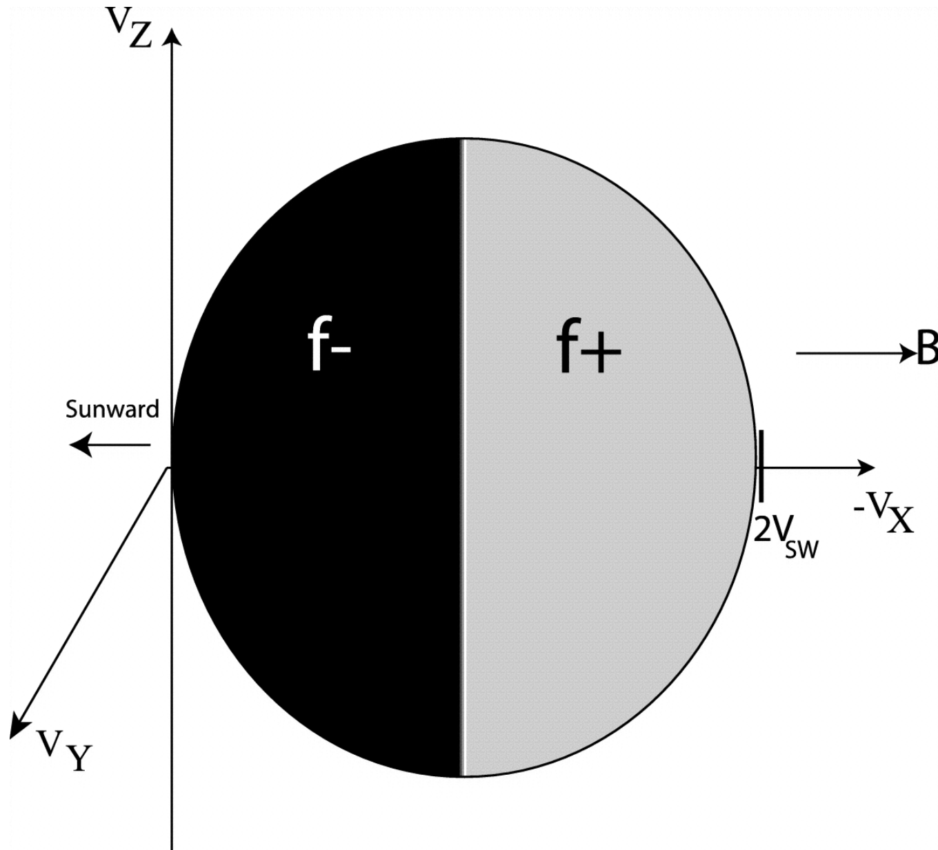
Fig. 4. from On PitchAngle Scattering Rates of Interstellar Pickup Ions as Determined by in Situ Measurement of Velocity Distributions Saul et al. 2007 ApJ 655 672 doi:10.1086/509732 https://dx.doi.org/10.1086/509732 © 2007. The American Astronomical Society. All rights reserved. Printed in U.S.A.
