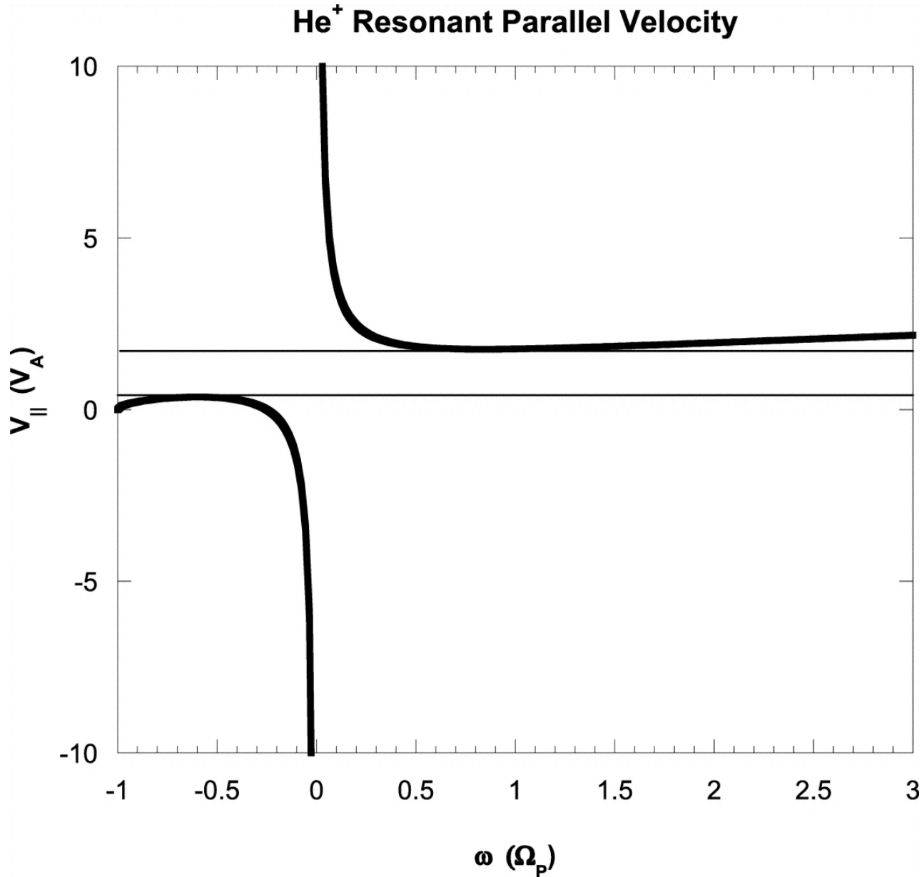
Fig. 3. from On PitchAngle Scattering Rates of Interstellar Pickup Ions as Determined by in Situ Measurement of Velocity Distributions Saul et al. 2007 ApJ 655 672 doi:10.1086/509732 https://dx.doi.org/10.1086/509732 © 2007. The American Astronomical Society. All rights reserved. Printed in U.S.A.
