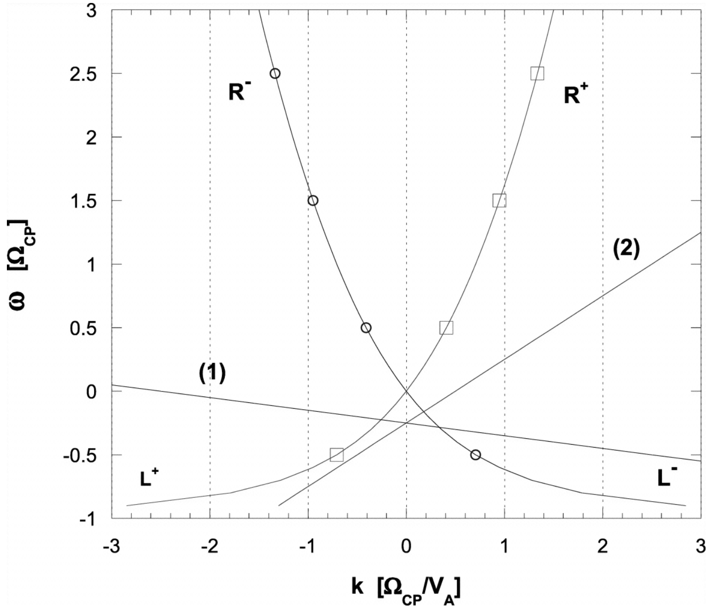
Fig. 2. from On PitchAngle Scattering Rates of Interstellar Pickup Ions as Determined by in Situ Measurement of Velocity Distributions Saul et al. 2007 ApJ 655 672 doi:10.1086/509732 https://dx.doi.org/10.1086/509732 © 2007. The American Astronomical Society. All rights reserved. Printed in U.S.A.
