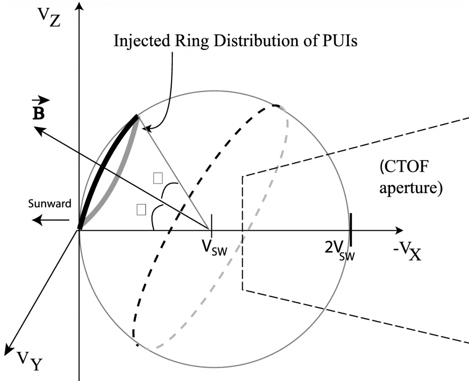
Fig. 1. from On PitchAngle Scattering Rates of Interstellar Pickup Ions as Determined by in Situ Measurement of Velocity Distributions Saul et al. 2007 ApJ 655 672 doi:10.1086/509732 https://dx.doi.org/10.1086/509732 © 2007. The American Astronomical Society. All rights reserved. Printed in U.S.A.
