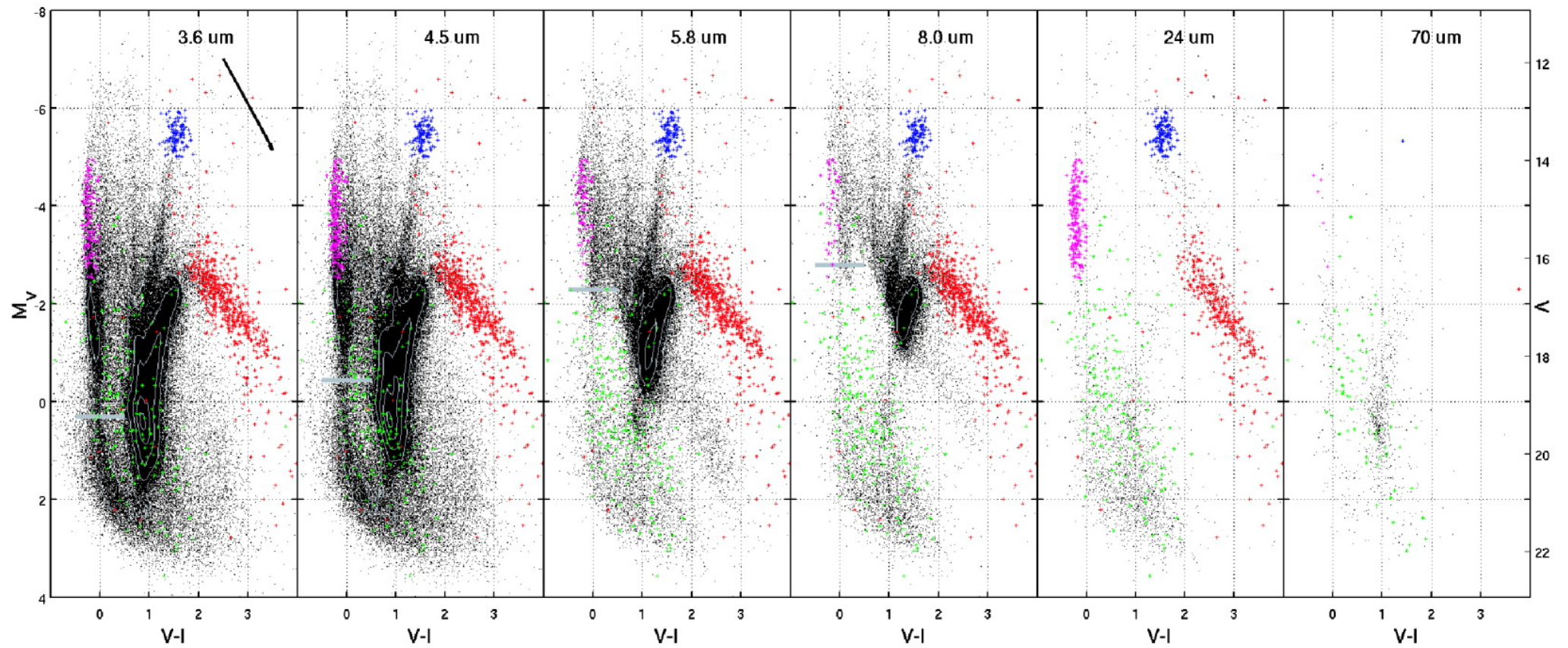
Fig. 9. from The Spitzer Survey of the Small Magellanic Cloud: S3MC Imaging and Photometry in the Mid and FarInfrared Wave Bands Bolatto et al. 2007 ApJ 655 212 doi:10.1086/509104 https://dx.doi.org/10.1086/509104 © 2007. The American Astronomical Society. All rights reserved. Printed in U.S.A.
