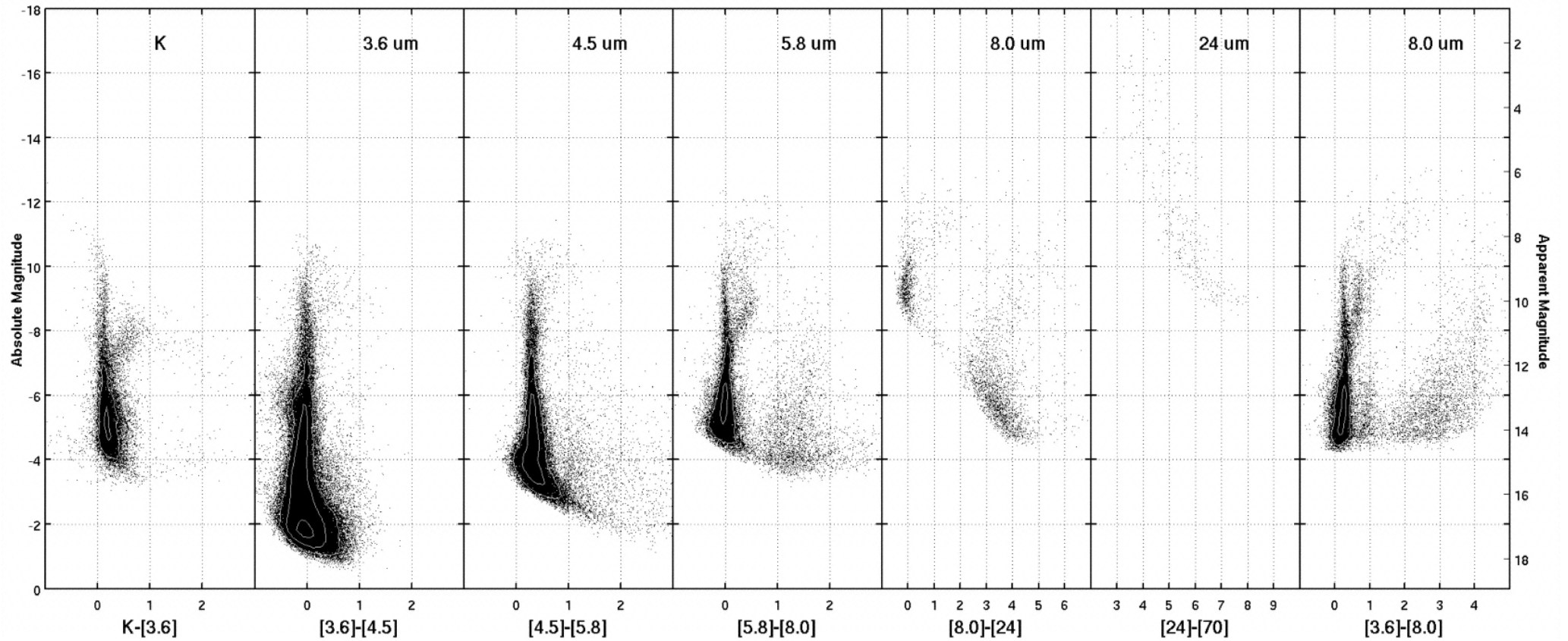
Fig. 8. from The Spitzer Survey of the Small Magellanic Cloud: S3MC Imaging and Photometry in the Mid and FarInfrared Wave Bands Bolatto et al. 2007 ApJ 655 212 doi:10.1086/509104 https://dx.doi.org/10.1086/509104 © 2007. The American Astronomical Society. All rights reserved. Printed in U.S.A.
