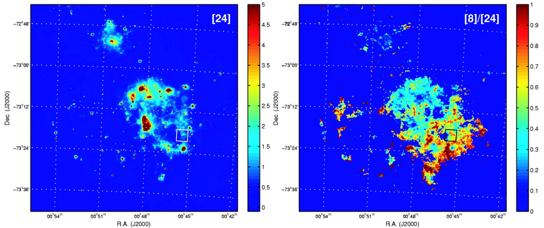
Fig. 5. from The Spitzer Survey of the Small Magellanic Cloud: S3MC Imaging and Photometry in the Mid and FarInfrared Wave Bands Bolatto et al. 2007 ApJ 655 212 doi:10.1086/509104 https://dx.doi.org/10.1086/509104 © 2007. The American Astronomical Society. All rights reserved. Printed in U.S.A.
