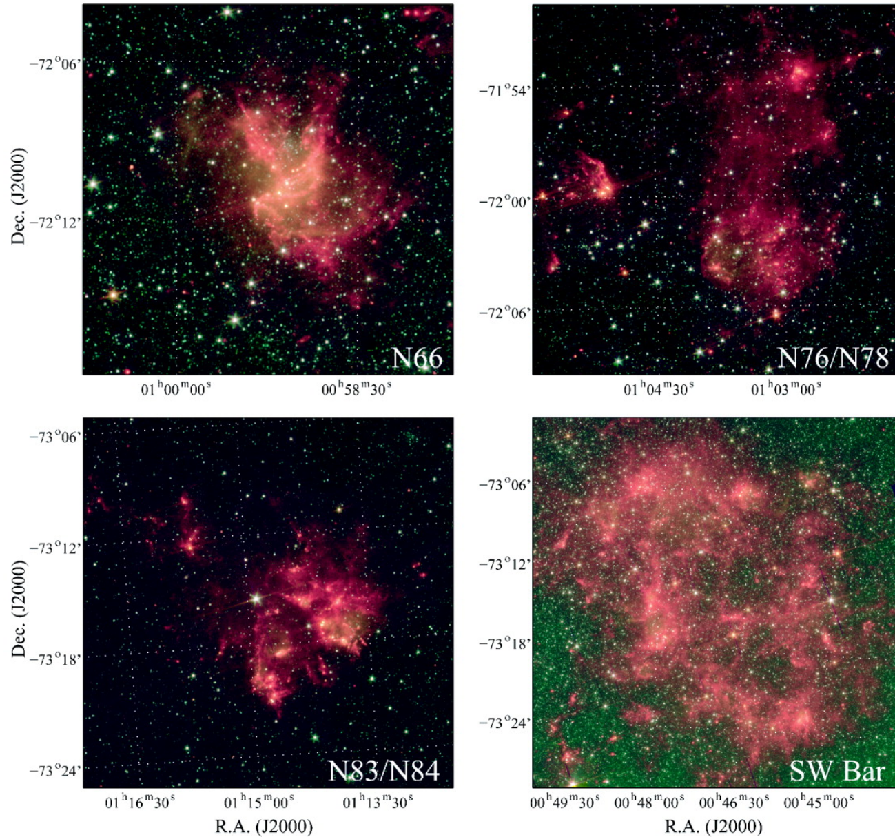
Fig. 4. from The Spitzer Survey of the Small Magellanic Cloud: S3MC Imaging and Photometry in the Mid and FarInfrared Wave Bands Bolatto et al. 2007 ApJ 655 212 doi:10.1086/509104 https://dx.doi.org/10.1086/509104 © 2007. The American Astronomical Society. All rights reserved. Printed in U.S.A.
