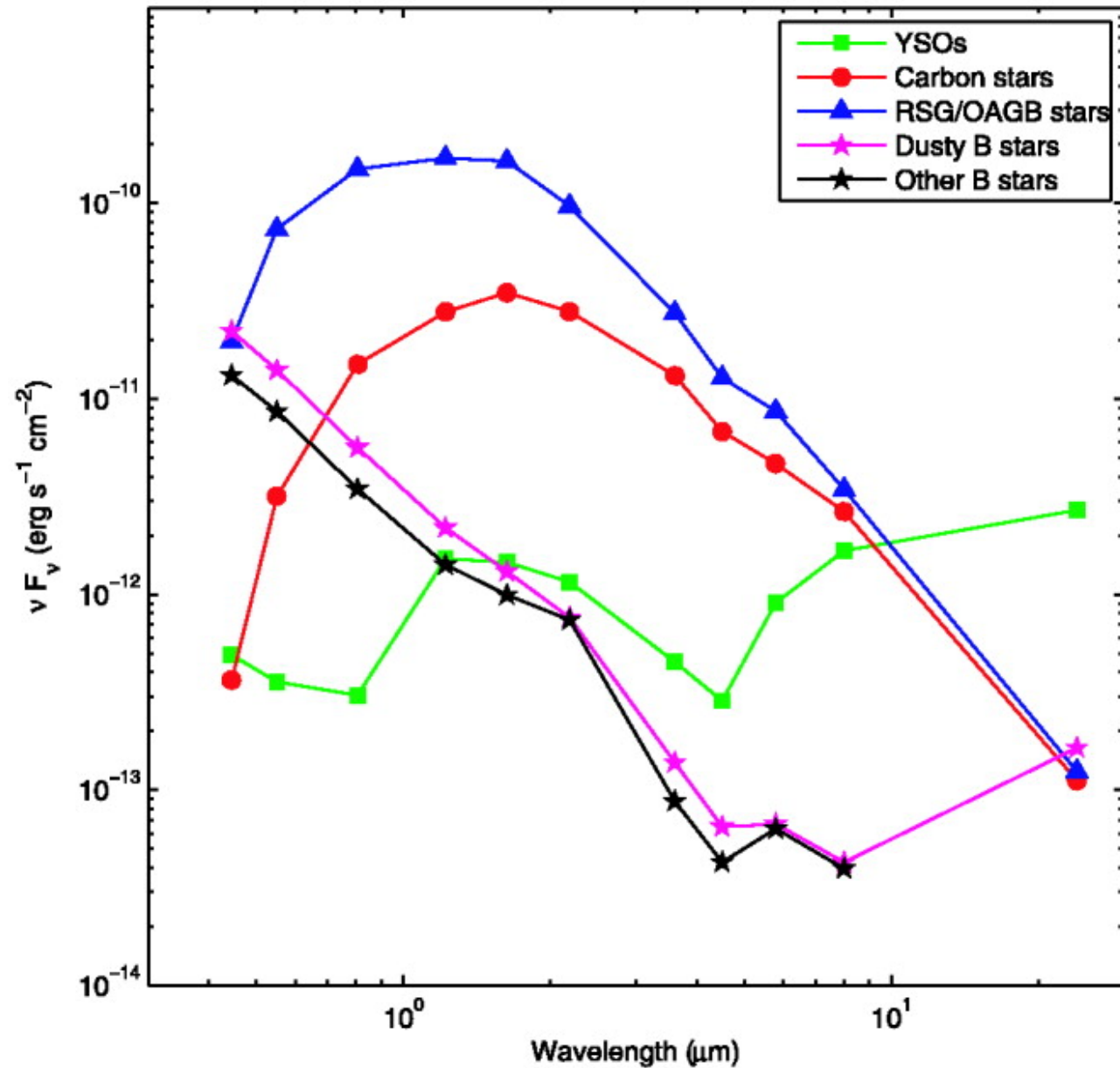
Fig. 13. from The Spitzer Survey of the Small Magellanic Cloud: S3MC Imaging and Photometry in the Mid and FarInfrared Wave Bands Bolatto et al. 2007 ApJ 655 212 doi:10.1086/509104 https://dx.doi.org/10.1086/509104 © 2007. The American Astronomical Society. All rights reserved. Printed in U.S.A.
