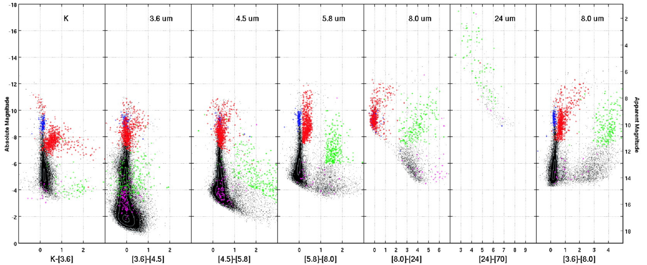
Fig. 10. from The Spitzer Survey of the Small Magellanic Cloud: S3MC Imaging and Photometry in the Mid and FarInfrared Wave Bands Bolatto et al. 2007 ApJ 655 212 doi:10.1086/509104 https://dx.doi.org/10.1086/509104 © 2007. The American Astronomical Society. All rights reserved. Printed in U.S.A.
