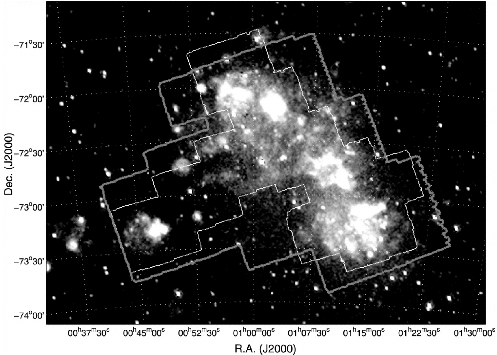
Fig. 1. from The Spitzer Survey of the Small Magellanic Cloud: S3MC Imaging and Photometry in the Mid and FarInfrared Wave Bands Bolatto et al. 2007 ApJ 655 212 doi:10.1086/509104 https://dx.doi.org/10.1086/509104 © 2007. The American Astronomical Society. All rights reserved. Printed in U.S.A.
