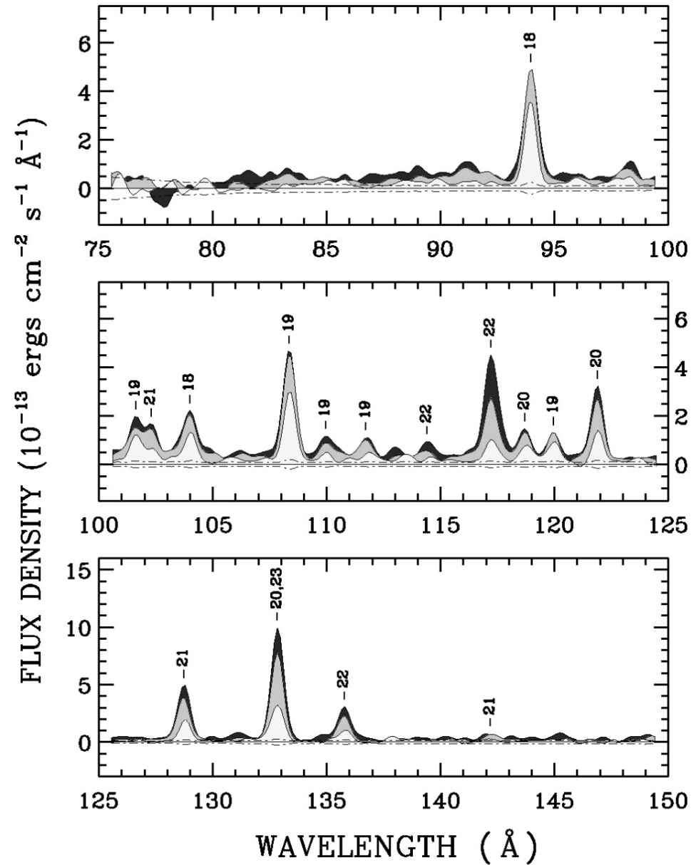
Fig. 2. from 3 Ms in the Life of Ceti: Sustained Flare Activity on a Clump Giant Detected by the Extreme Ultraviolet Explorer Ayres, Osten, & Brown 2001 ApJL 562 L83 doi:10.1086/337971 https://dx.doi.org/10.1086/337971
