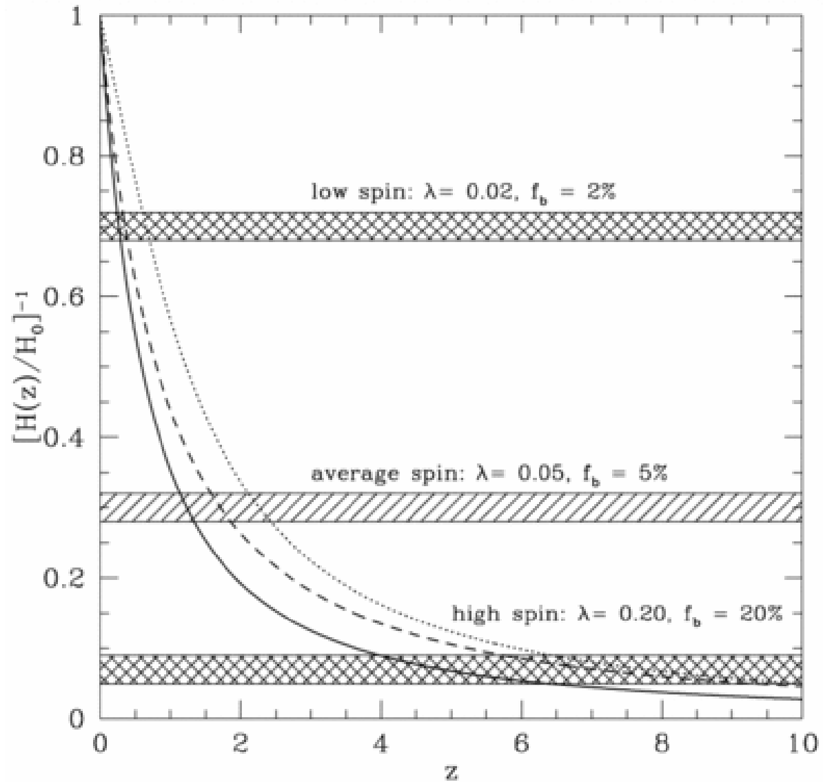
Fig. 1. from Consequences of Feedback from Early Supernovae for Disk Assembly Natarajan 1999 ApJL 512 L105 doi:10.1086/311877 https://dx.doi.org/10.1086/311877 © 1999. The American Astronomical Society. All rights reserved. Printed in U.S.A.
