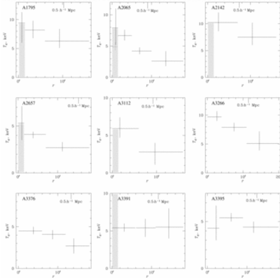
Fig. 4. from The Temperature Structure of 30 Nearby Clusters Observed with ASCA: Similarity of Temperature Profiles Temperature Structure of Clusters 1998 ApJ 503 77 doi:10.1086/305976 https://dx.doi.org/10.1086/305976 © 1998. The American Astronomical Society. All rights reserved. Printed in U.S.A.
