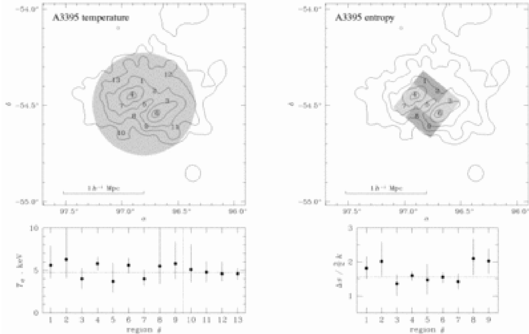
Fig. 3. from The Temperature Structure of 30 Nearby Clusters Observed with ASCA: Similarity of Temperature Profiles Temperature Structure of Clusters 1998 ApJ 503 77 doi:10.1086/305976 https://dx.doi.org/10.1086/305976 © 1998. The American Astronomical Society. All rights reserved. Printed in U.S.A.
