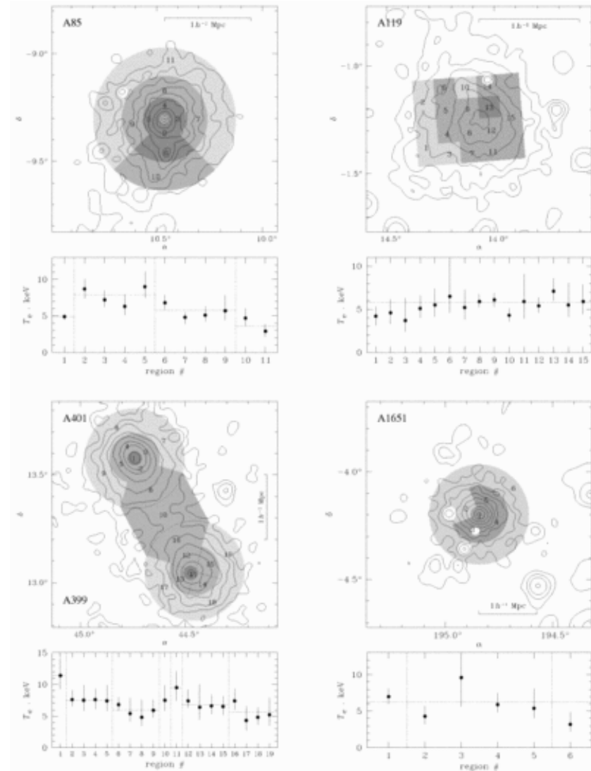
Fig. 2. from The Temperature Structure of 30 Nearby Clusters Observed with ASCA: Similarity of Temperature Profiles Temperature Structure of Clusters 1998 ApJ 503 77 doi:10.1086/305976 https://dx.doi.org/10.1086/305976 © 1998. The American Astronomical Society. All rights reserved. Printed in U.S.A.
