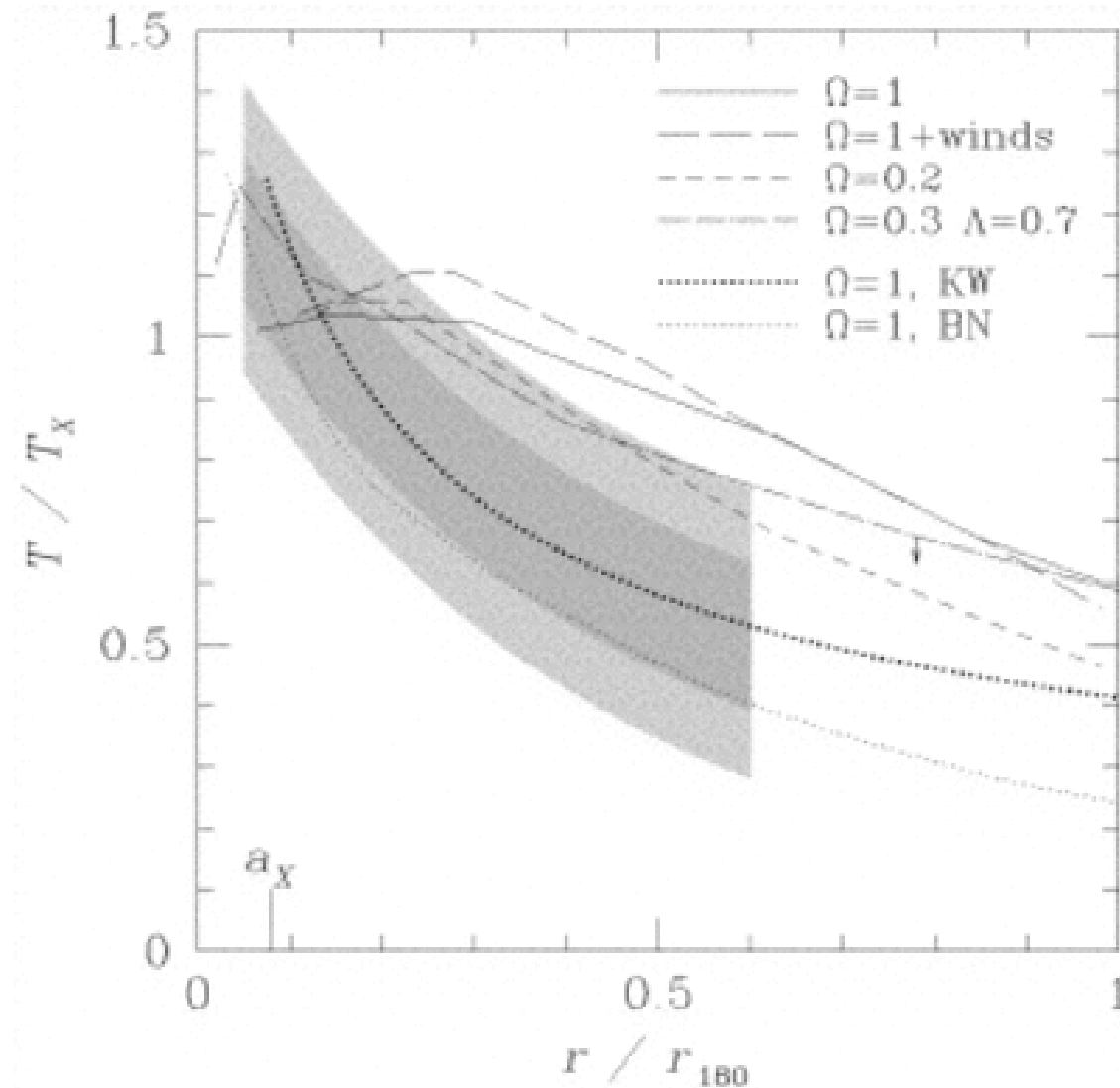
Fig. 8. from The Temperature Structure of 30 Nearby Clusters Observed with ASCA: Similarity of Temperature Profiles Temperature Structure of Clusters 1998 ApJ 503 77 doi:10.1086/305976 https://dx.doi.org/10.1086/305976 © 1998. The American Astronomical Society. All rights reserved. Printed in U.S.A.
