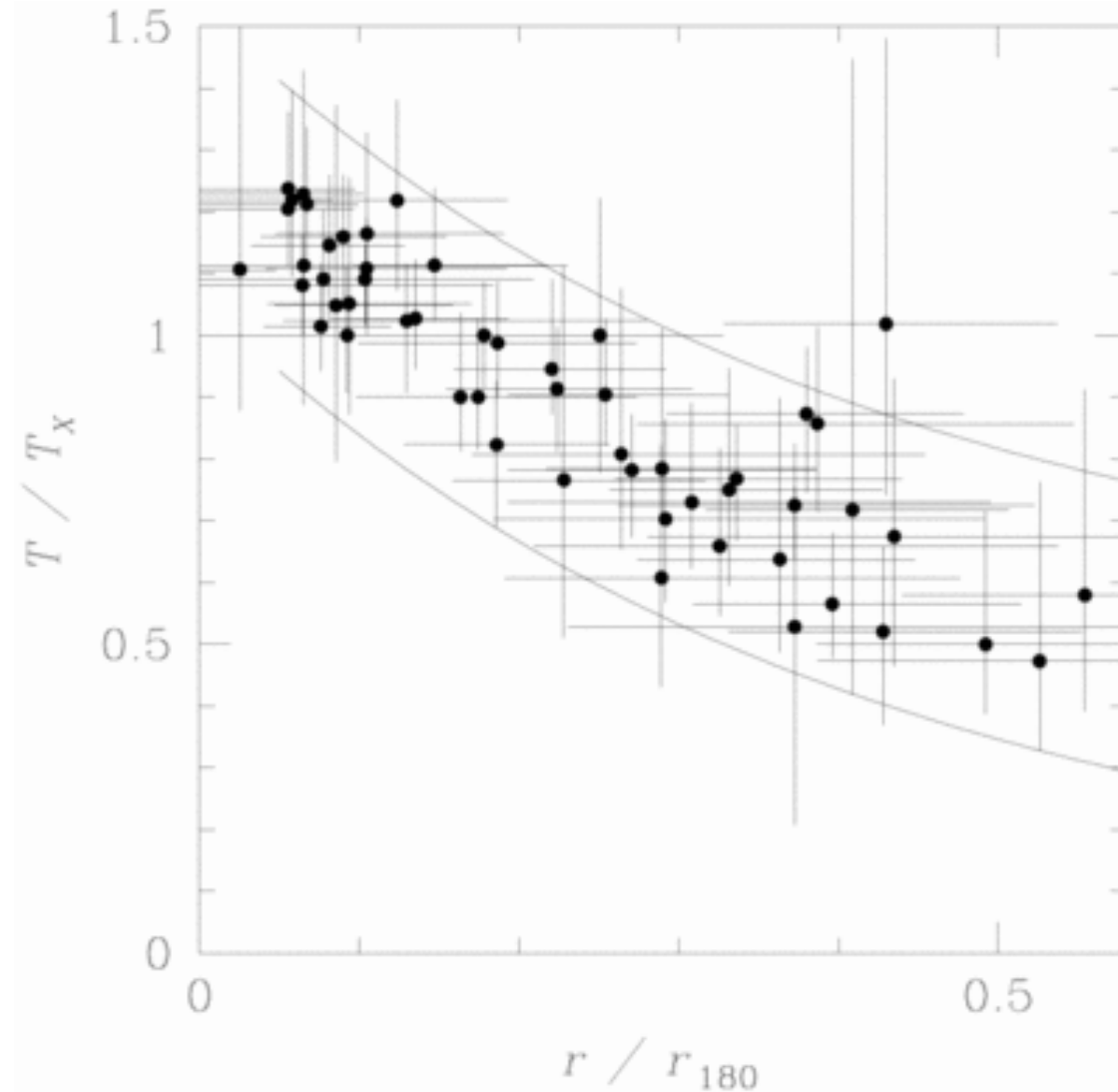
Fig. 7. from The Temperature Structure of 30 Nearby Clusters Observed with ASCA: Similarity of Temperature Profiles Temperature Structure of Clusters 1998 ApJ 503 77 doi:10.1086/305976 https://dx.doi.org/10.1086/305976 © 1998. The American Astronomical Society. All rights reserved. Printed in U.S.A.
