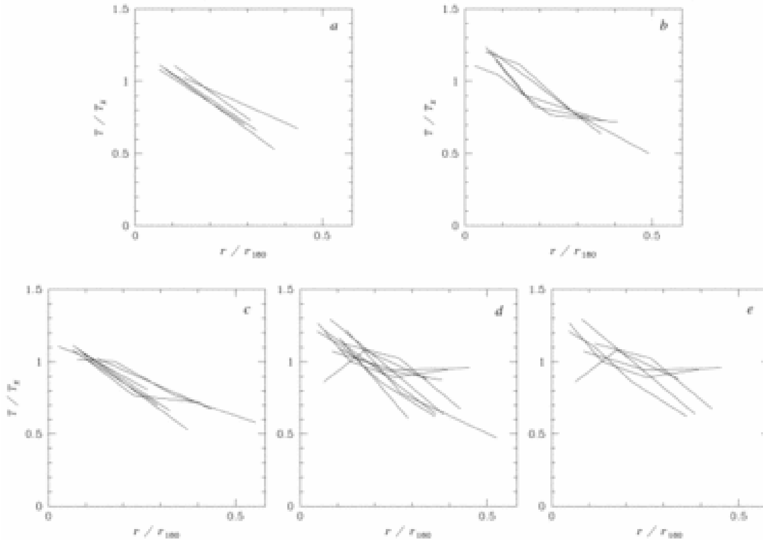
Fig. 6. from The Temperature Structure of 30 Nearby Clusters Observed with ASCA: Similarity of Temperature Profiles Temperature Structure of Clusters 1998 ApJ 503 77 doi:10.1086/305976 https://dx.doi.org/10.1086/305976 © 1998. The American Astronomical Society. All rights reserved. Printed in U.S.A.
