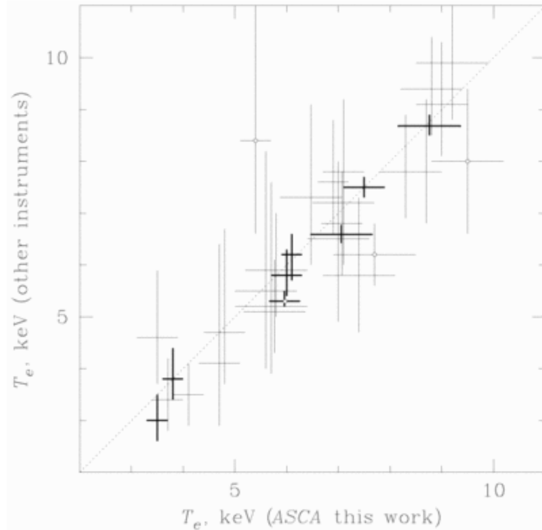
Fig. 1. from The Temperature Structure of 30 Nearby Clusters Observed with ASCA: Similarity of Temperature Profiles Temperature Structure of Clusters 1998 ApJ 503 77 doi:10.1086/305976 https://dx.doi.org/10.1086/305976 © 1998. The American Astronomical Society. All rights reserved. Printed in U.S.A.
