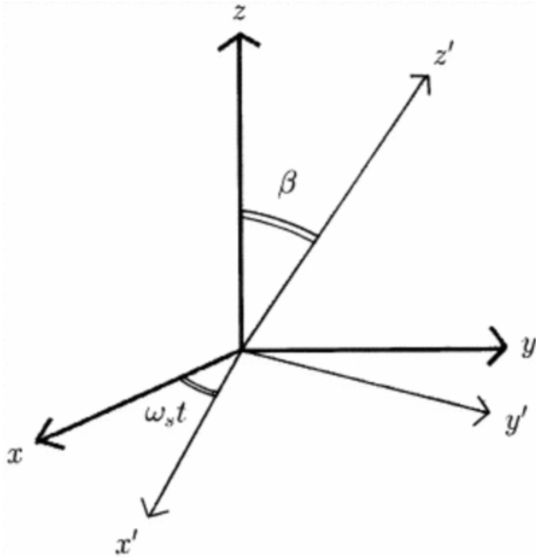
Fig. 2. from A New Instability of Accretion Disks around Magnetic Compact Stars Vietri & Stella 1998 ApJ 503 350 doi:10.1086/305970 https://dx.doi.org/10.1086/305970 © 1998. The American Astronomical Society. All rights reserved. Printed in U.S.A.
